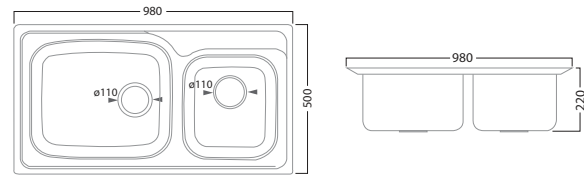
CKS9850 Dimension : L980xW500xH220mm List Price : RM 1,650
