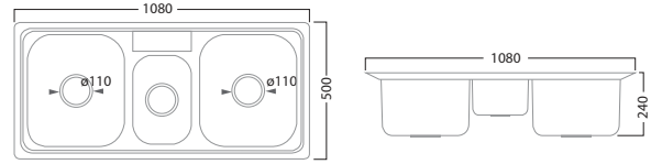
CKS1080-BL Dimension : L1080xW500xH240mm Color : Matt Black List Price : RM 935
