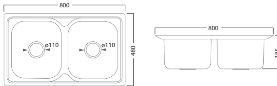
CKS8048 Dimension : L800xW480xH185mm List Price : RM 277
